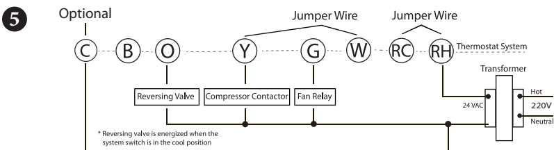
Typical Wiring Diagram For Heat Pump With Reversing Valve Energized In Cool
